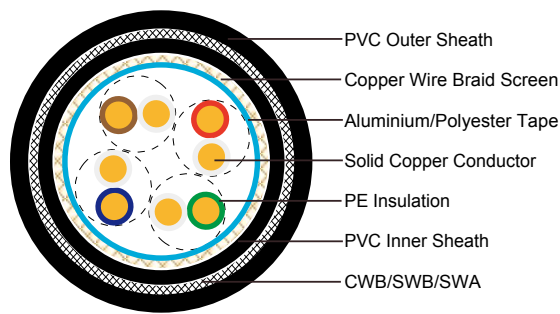
SF/UTP CAT6
