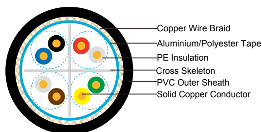
SF/UTP CAT6
